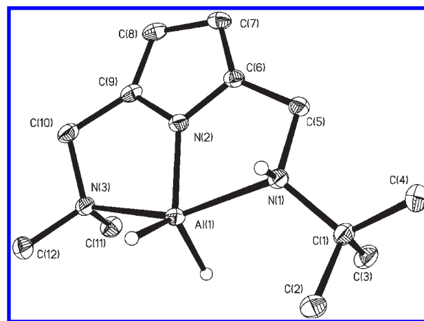
Figure 2. Molecular structure of 2 . The thermal ellipsoids are shown at the 30% probability level. All of the hydrogen atoms are omitted for clarity.
