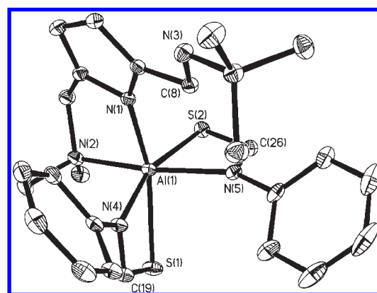
Figure 4. Molecular structure of 4. The thermal ellipsoids are shown at the 30% probability level. All of the diethyl ether and hydrogen atoms are omitted for clarity.
