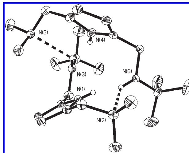
Figure 1. Molecular structure of 1 . The thermal ellipsoids are shown at the 30% probability level. All of the hydrogen atoms (except NH) are omitted for clarity.
