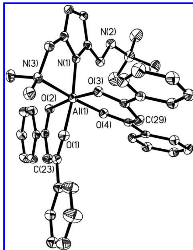
Figure 3. Molecular structure of 3. The thermal ellipsoids are shown at the 30% probability level. All of the toluene and hydrogen atoms are omitted for clarity.
